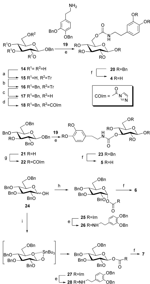
Scheme 1 (a) TrCl (1.5 equiv), DMAP (0.2 equiv), pyridine, 60^\circ C ; (b) BnBr (3.3 equiv), NaH (3.7 equiv), DMF ; (c) p-TsOH (0.2 equiv), CH_2Cl_2 - MeOH ; (d) N,N -carbonyldiimidazole (1.2 equiv), dioxane; (e) 19 (0.85 equiv), Et_3N , THF , 80^\circ C ; (f) H_2 , Pd/C , AcOEt - MeOH -toluene 4 : 3 : 3; (g) N,N -carbonyldiimidazole (1.2 equiv), THF ; (h) N,N -carbonyldiimidazole, Et_2O ; (i) (Bu_3Sn)_2 (1 equiv), toluene, 120^\circ C , 2 h, then, N,N -carbonyldiimidazole (2 equiv), rt .
