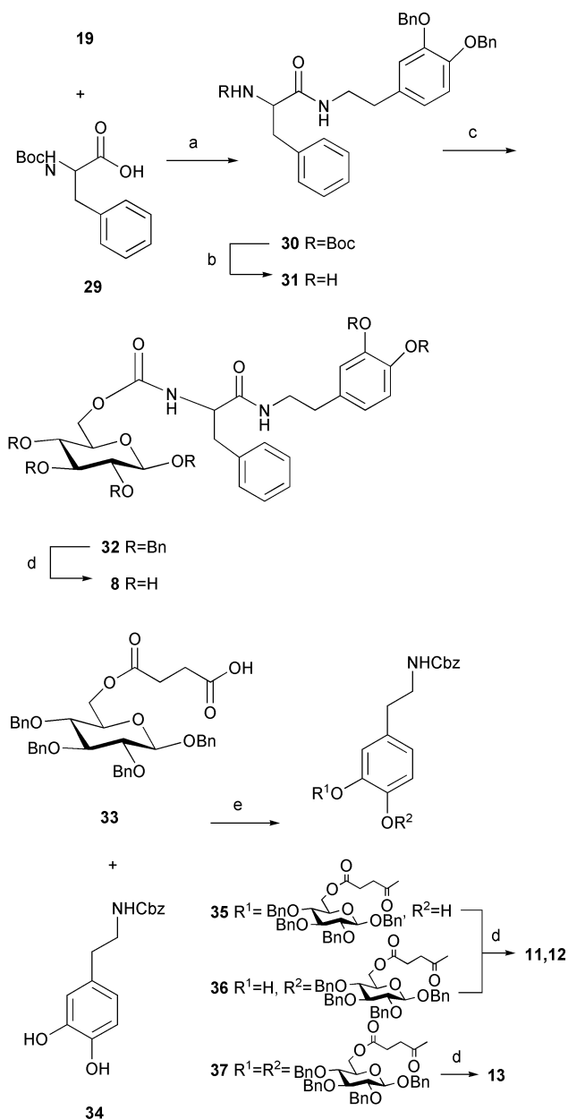
Scheme 2 (a) 19 (1 equiv), 29 (1 equiv), Et_3N (4 equiv), BOP (1.1 equiv), THF ; (b) TFA , CH_2Cl_2 ; (c) 18 (1.2 equiv), Et_3N , THF , 80^\circ C ; (d) H_2 , Pd/C , AcOEt - MeOH -toluene 4 : 3 : 3; (e) 33 (1 equiv), 34 (0.66 equiv), diisopropylcarbodiimide ( DIIC ) (1.3 equiv), CH_2Cl_2 .
